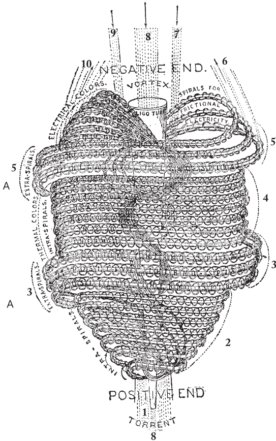
Fig 135. The general Form of an Atom, including the spirals and 1st Spirillae, together with influx and efflux ethers, represented by dots, which pass through these spirillae. The 2nd and 3rd spirillae and their still finer ethers are not shown.
